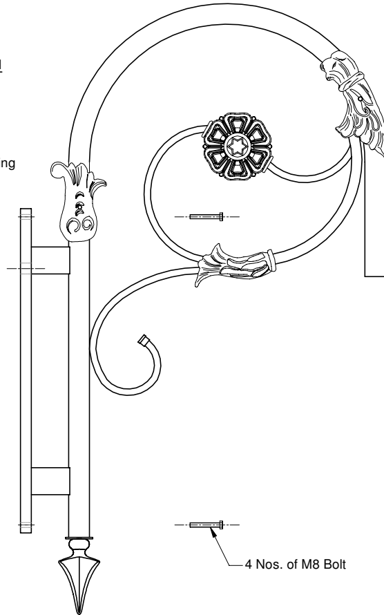
Mounting Detail Scale: 1.5 : 1
